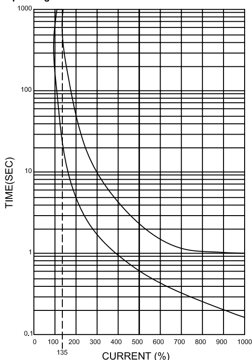
Operating Characteristics :
