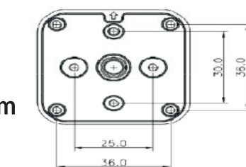
Switch Mounting Details 8 holes - for self threading screw - M3x9 mm
