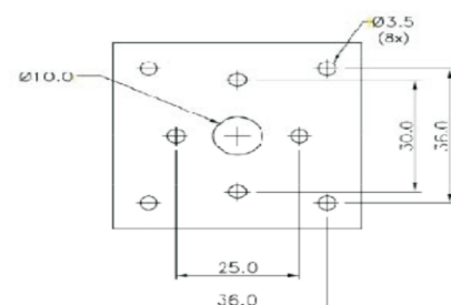
Drilling Plan
